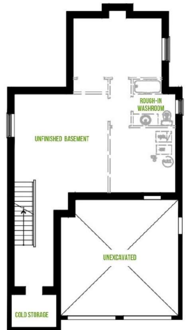
Basement Plan
