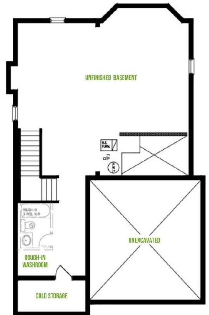
Basement Plan
